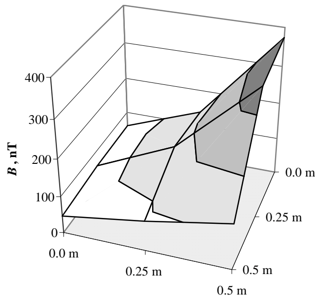
Figure 3: EMF (50 Hz) levels distribution (B-field)
