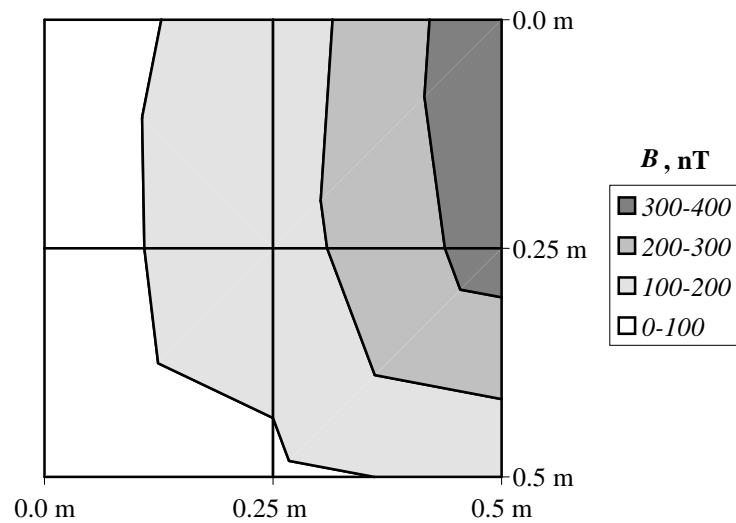
Figure 2: RF EMF levels distribution (E-field) at 1714 MHz
